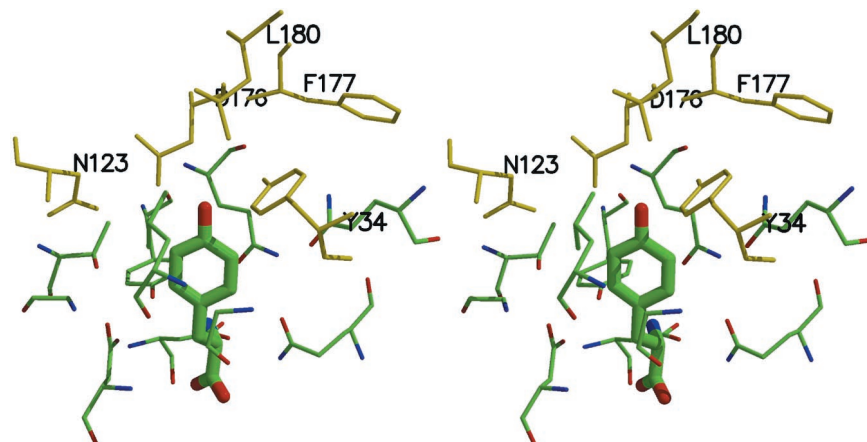
Fig. 1. Stereo view of the active site of TyrRS (18). Residues from B. stearrowtherophilus TyrRS are shown in the figure. Corresponding residues from M. jannaschii TyrRS are Tyr 32 (Tyr 34 ), Glu 107 (Asn 123 ), Asp 158 (Asp 176 ), Ile 159 (Phe 177 ), and Leu 162 (Leu 180 ) with residues from B. stearrowtherophilus TyrRS in parenthesis; mutated residues are in yellow.
