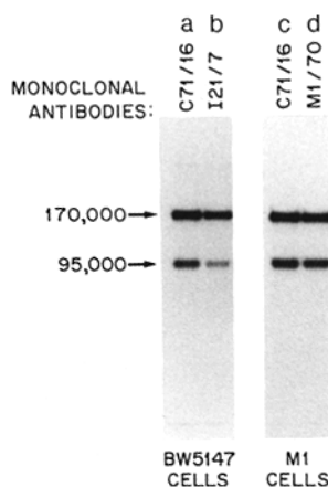
FIG. 2. SDS-polyacrylamide gel analysis of the labeled polypeptides precipitated by M1/70, C71/16, and I21/7 monoclonal antibodies from lysates of ^{125}\text{I} -labeled BW5147 cells and dexamethasone-induced M1 cells.
