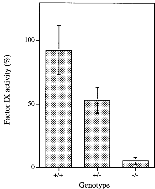
FIG. 3. Factor IX coagulant activity in FIX +/+ , +/- , and -/- mice. Factor IX activity was quantitated by using APTT assays. The factor IX activity for wild-type ( +/+ ) mice was 92.1 \pm 19.1\% ( n = 21 ), for heterozygous ( +/- ) mice was 52.9 \pm 10.4\% ( n = 12 ), and for homozygous ( -/- ) mice was 5.4 \pm 2.9\% ( n = 26 ).
